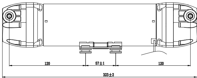
LFP2200W-FD - LFP22600W-FD (3/8" SIDE FEMALE QUICK CONNECTOR)
