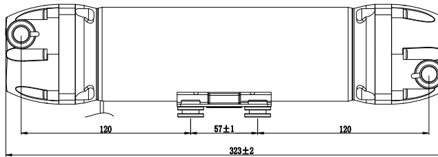
LFP2200W-FD - LFP22600W-FD (3/8" NPT "0" )
